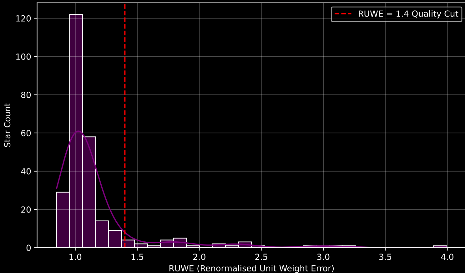
GALAH DR4 Field [1145] RUWE Distribution (n= 261)
