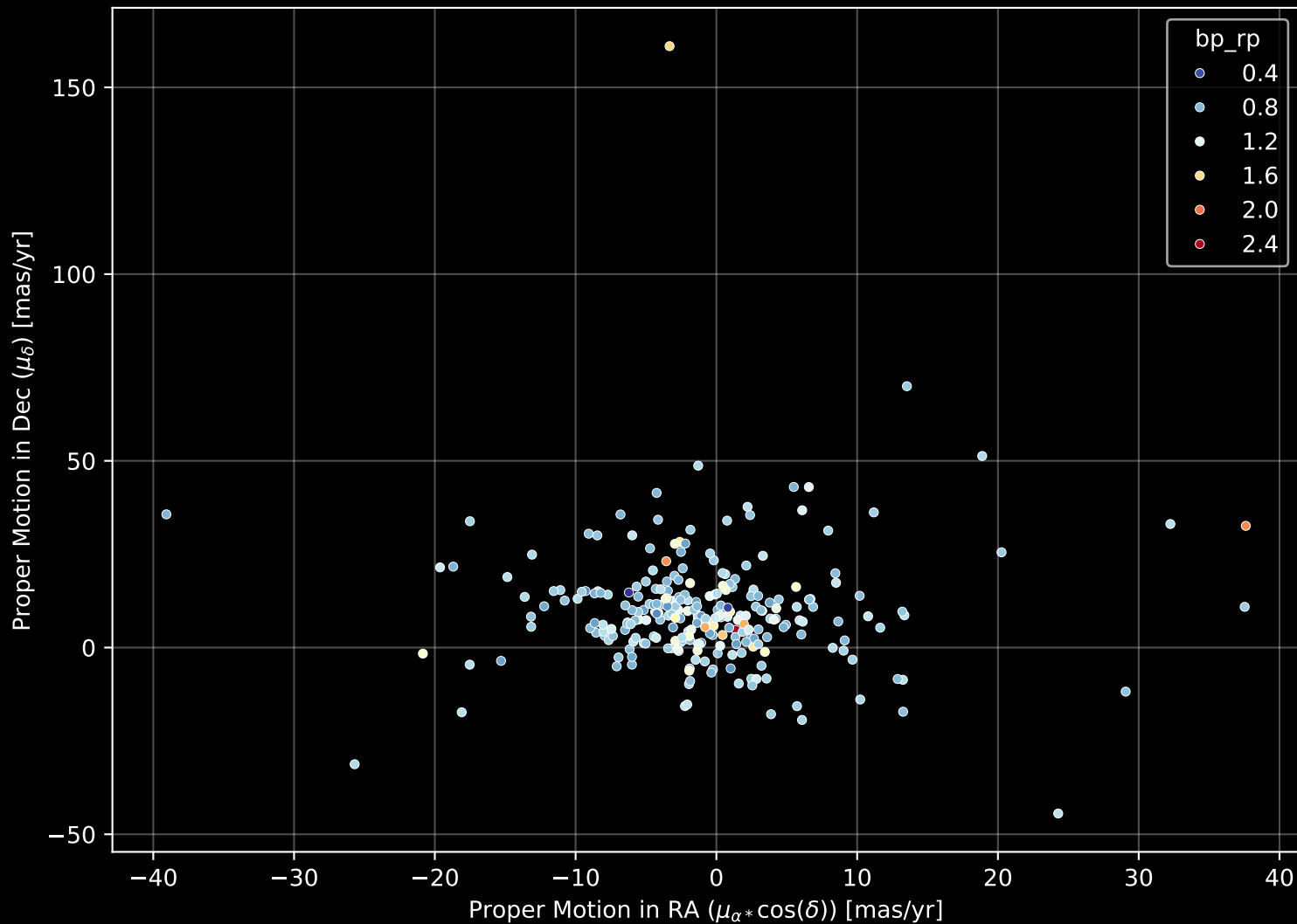
GALAH DR4 Field: [1145] Proper Motion Diagram (n= 269)
