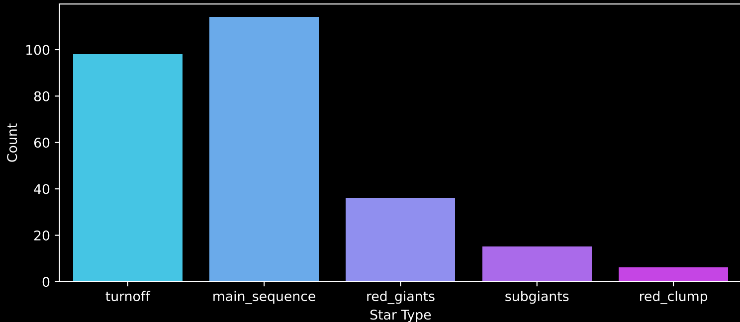
GALAH DR4 Field: [1145] Count plot of Star Type
